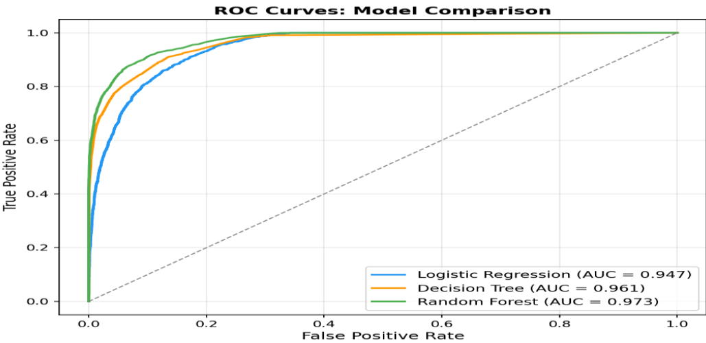
Figure 6.13: ROC curves for all three models. Random Forest achieves the highest AUC of 0.973.
