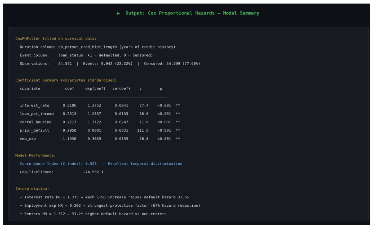
Output 6.16: Console output — Cox PH model summary with hazard ratios and concordance index ( C = 0.927 ).
